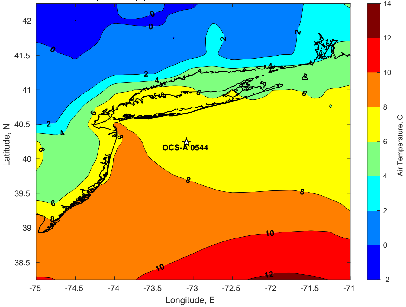
Air Temperature (C) for OCS-A 0544 at 20-Mar-2024
